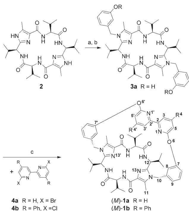
Scheme 2. Preparation of the chiral molecular hinges ( M )- 1 . Reaction conditions: a) 3-methoxybenzyl bromide, \text{Cs}_2\text{CO}_3 , \text{CH}_3\text{CN} , \Delta , 66%; b) \text{BBr}_3 , \text{CH}_2\text{Cl}_2 , -78^\circ\text{C} \rightarrow \text{RT} , 95%; c) \text{Cs}_2\text{CO}_3 , DMF, 110^\circ\text{C} , 20% for ( M )- 1a and 25% for ( M )- 1b .
