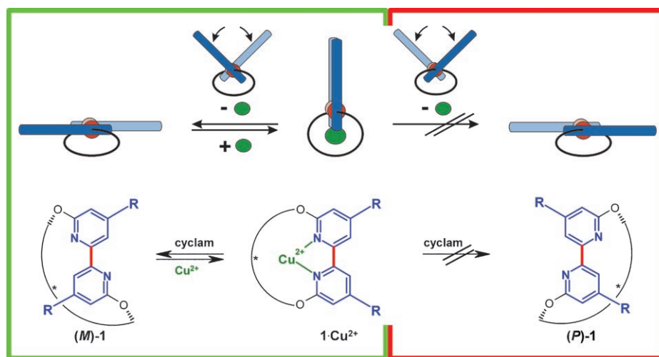
Scheme 1. Schematic representation of the chiral molecular hinge 1 and its unidirectional open–close motion.
