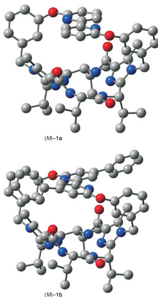
Figure 1. Molecular structures of ( M )- 1a and ( M )- 1b calculated using B3LYP/6-31G*. All hydrogen atoms have been omitted for clarity.
