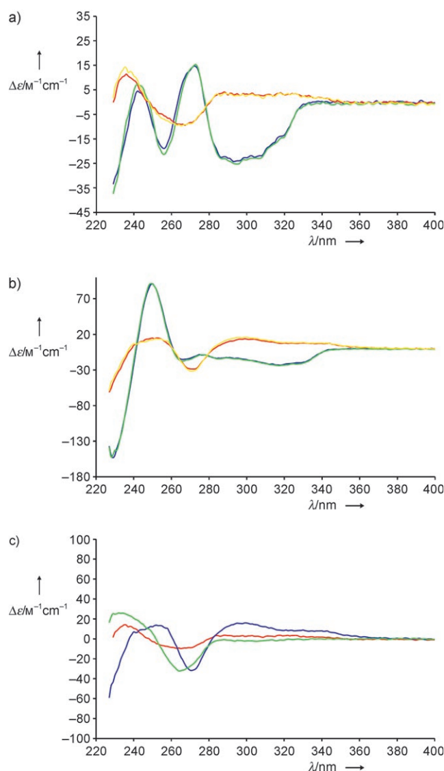
Figure 2. a) CD spectra of 1a (blue) with 2.5 (red) and 3.0 (yellow) equiv Cu(OTf) 2 and with 3.0 equiv Cu(OTf) 2 plus 6.0 equiv cyclam (green) ([ 1a ] = 1.0 × 10 −5 M in dichloromethane). b) CD spectra of 1b (blue) with 2.5 (red) and 3.0 (yellow) equiv Cu(OTf) 2 and with 3.0 equiv Cu(OTf) 2 plus 6.0 equiv cyclam (green) ([ 1b ] = 1.0 × 10 −5 M in dichloromethane). c) CD spectra of 1a (red), 1b (blue), and 3b (R = Me; green) each with 3.0 equiv Cu(OTf) 2 (c = 1.0 × 10 −5 M in dichloromethane).
